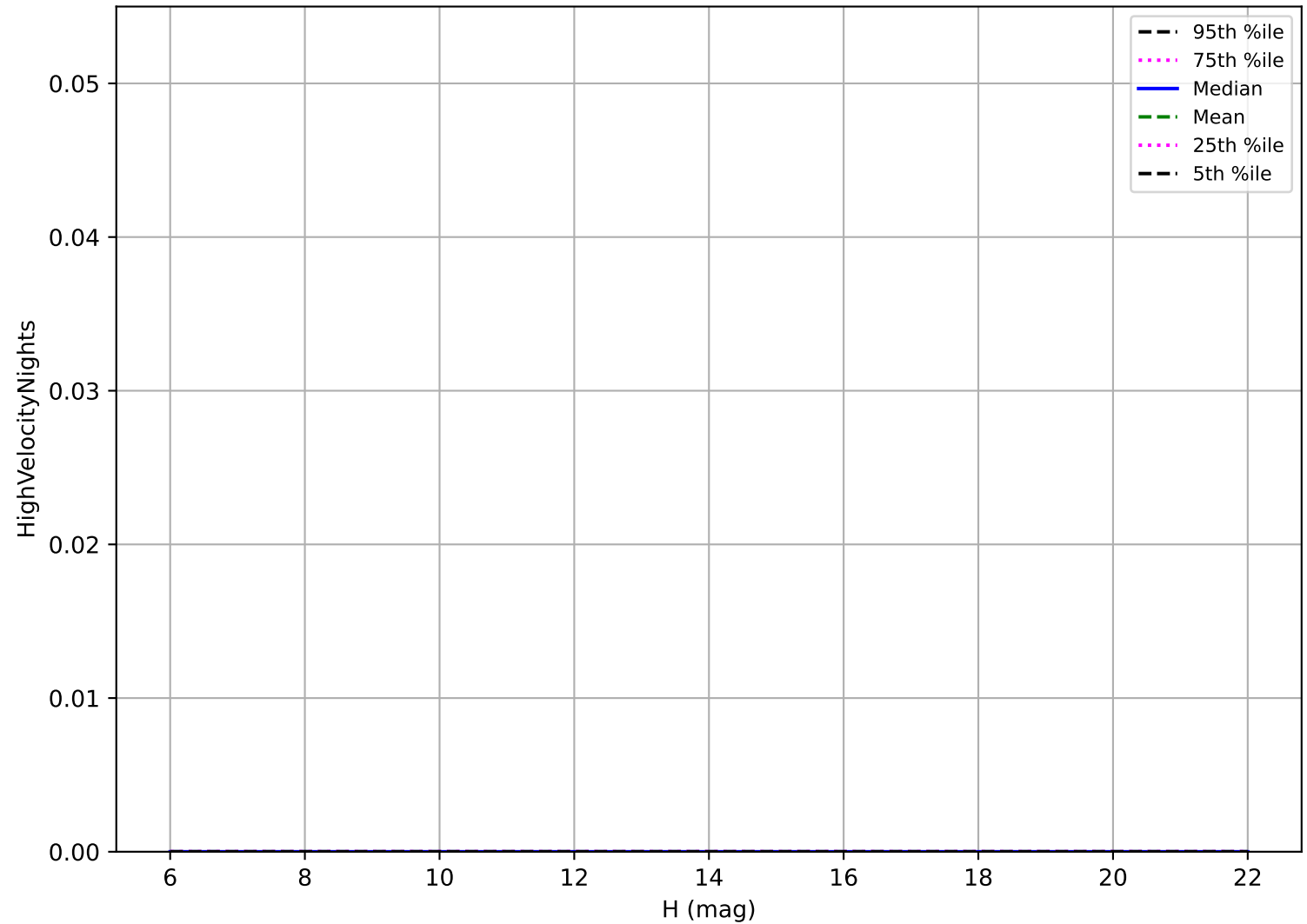
too_elab_r256_d3_giz_v3.4_10yrs: OCC_r5 High velocity pair detection loss
