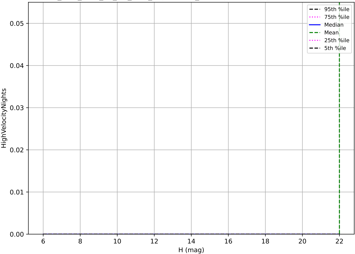
too_elab_r256_d3_giz_v3.4_10yrs: OCC_r20 High velocity pair detection loss
