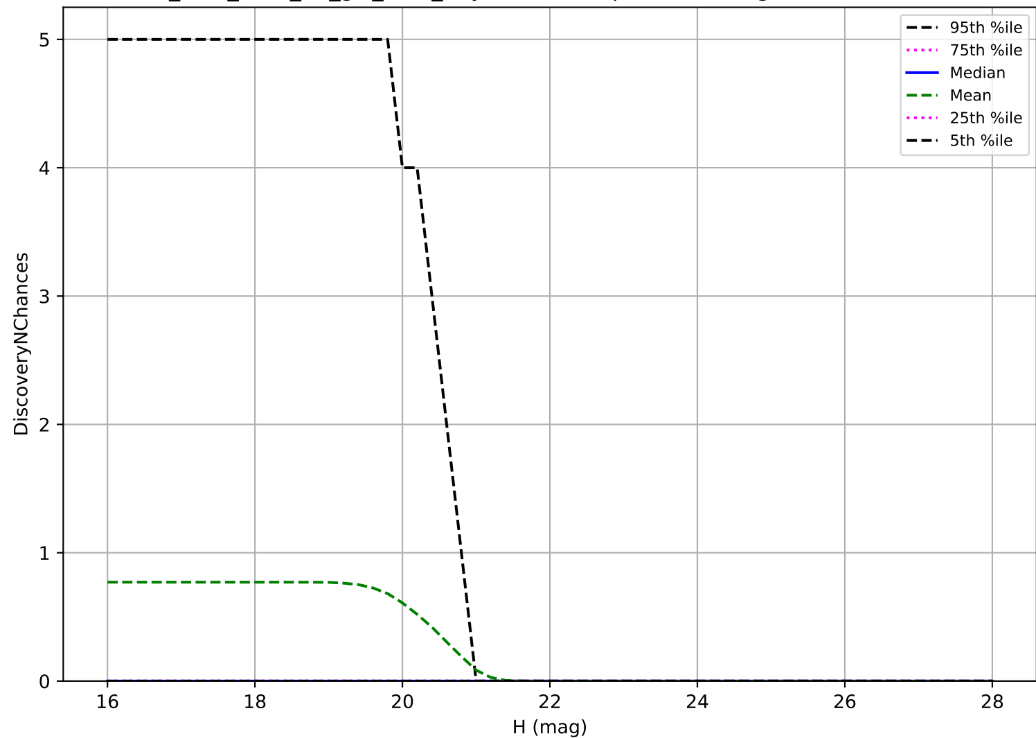
too_elab_r256_d3_giz_v3.4_10yrs: Vatira 3 pairs in 15 nights detection loss
