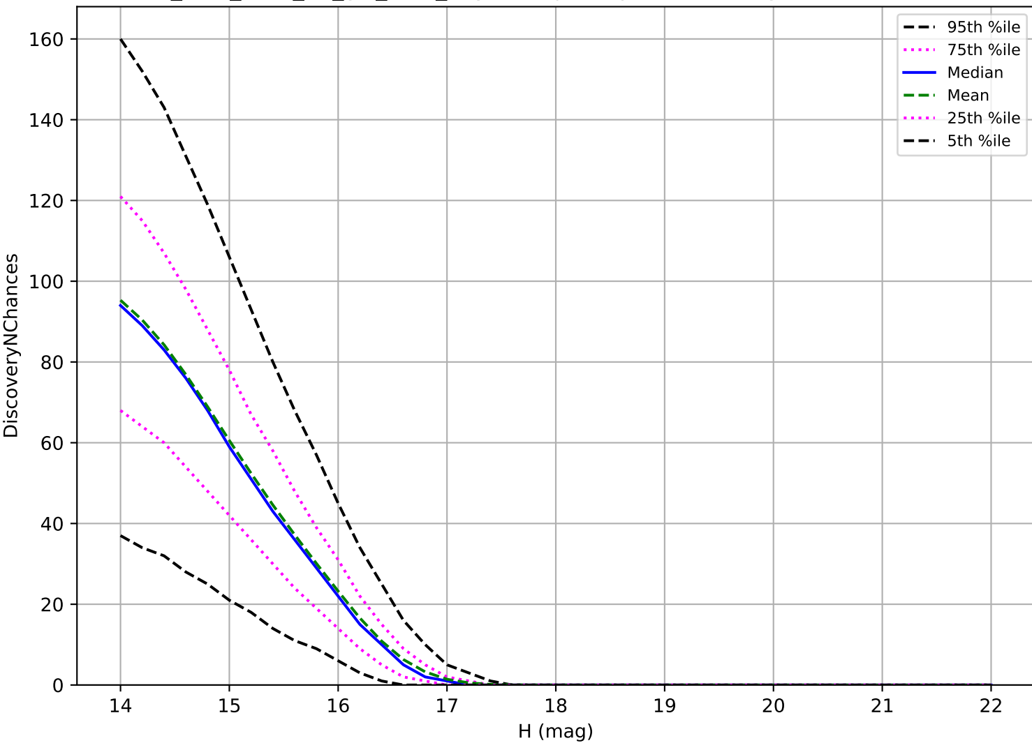
too_elab_r256_d3_giz_v3.4_10yrs: Trojan 3 pairs in 15 nights detection loss
