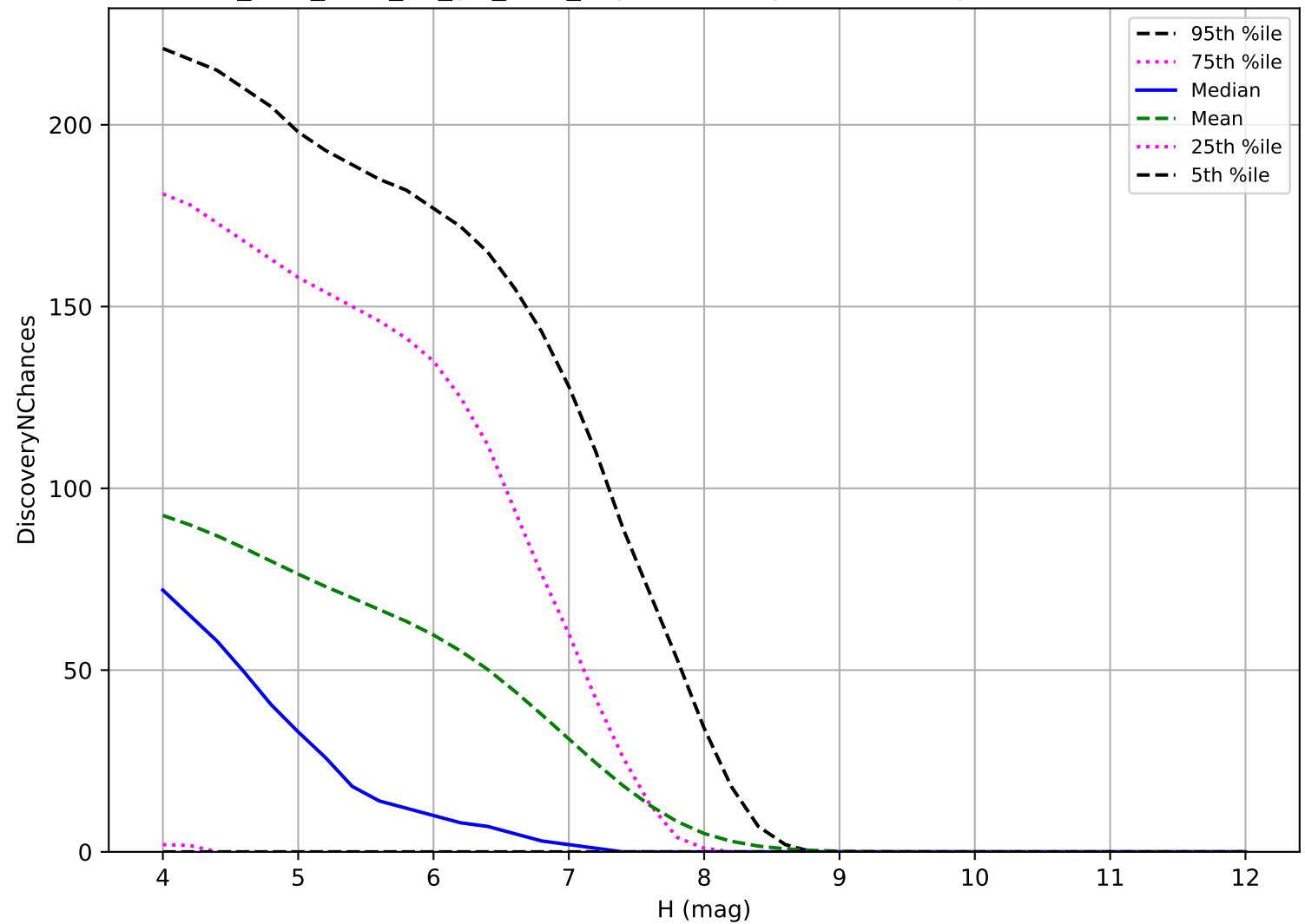
too_elab_r256_d3_giz_v3.4_10yrs: TNO 3 pairs in 15 nights detection loss
