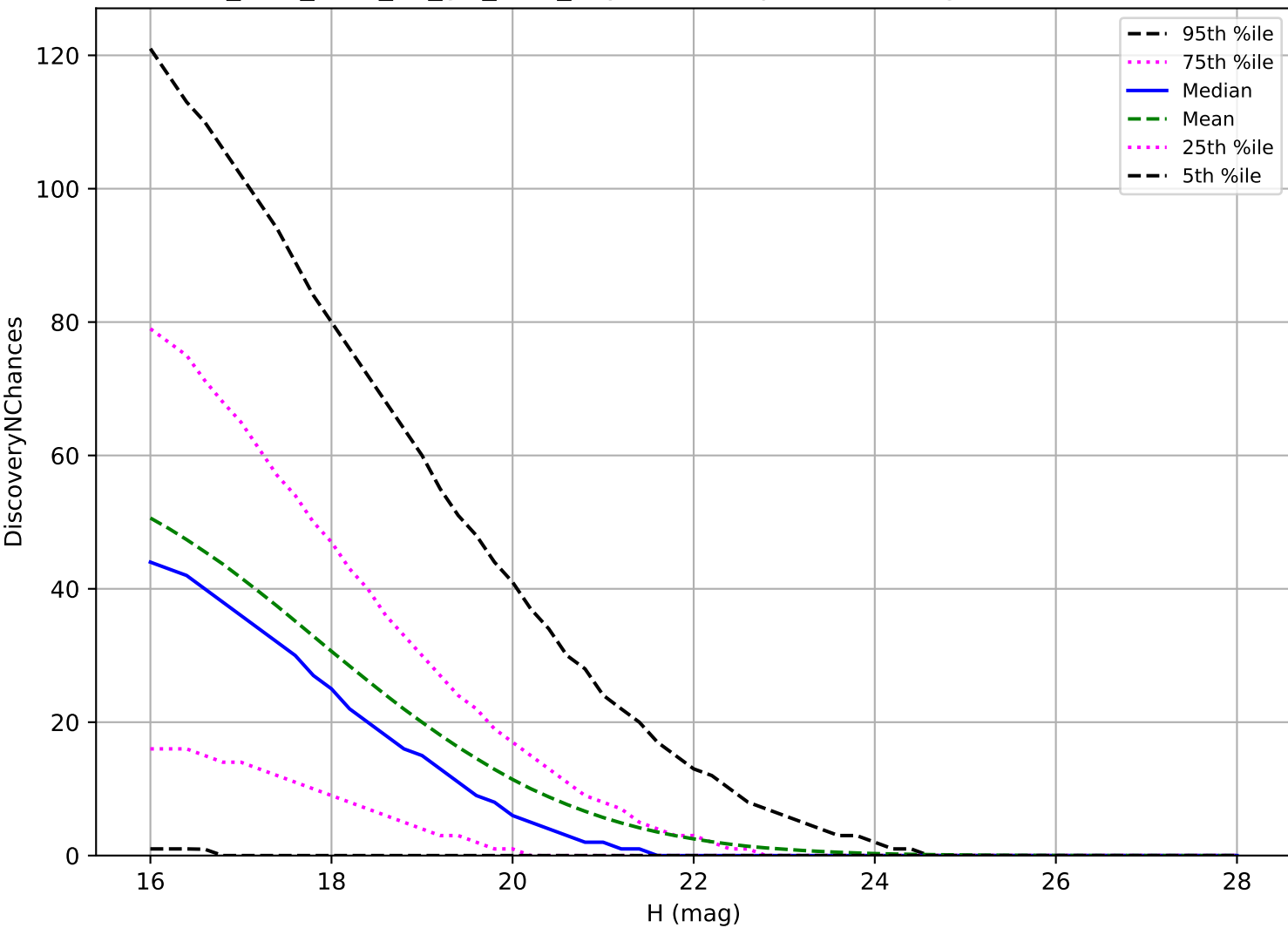
too_elab_r256_d3_giz_v3.4_10yrs: PHA 3 pairs in 15 nights detection loss
