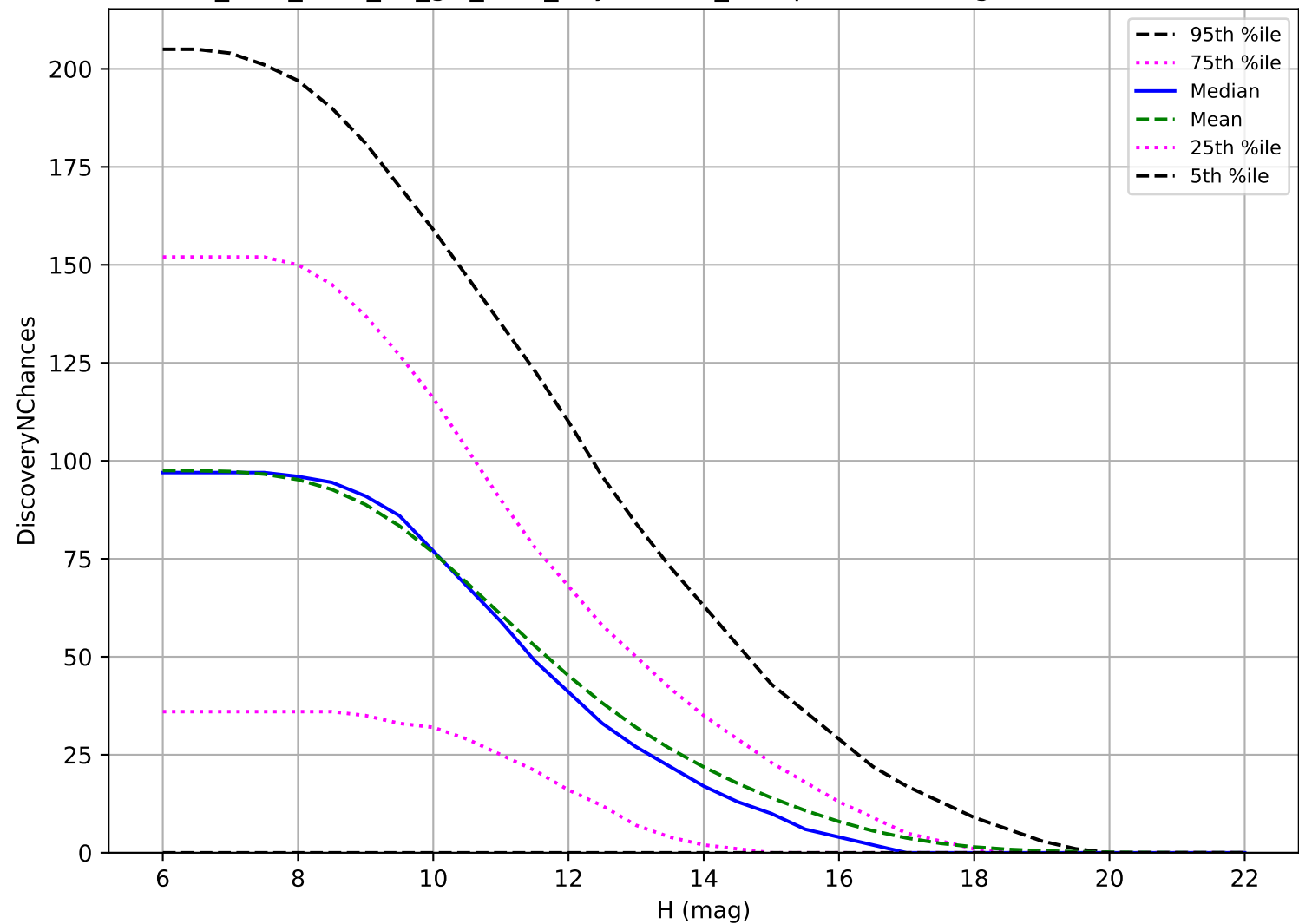
too_elab_r256_d3_giz_v3.4_10yrs: OCC_r5 3 pairs in 15 nights detection loss
