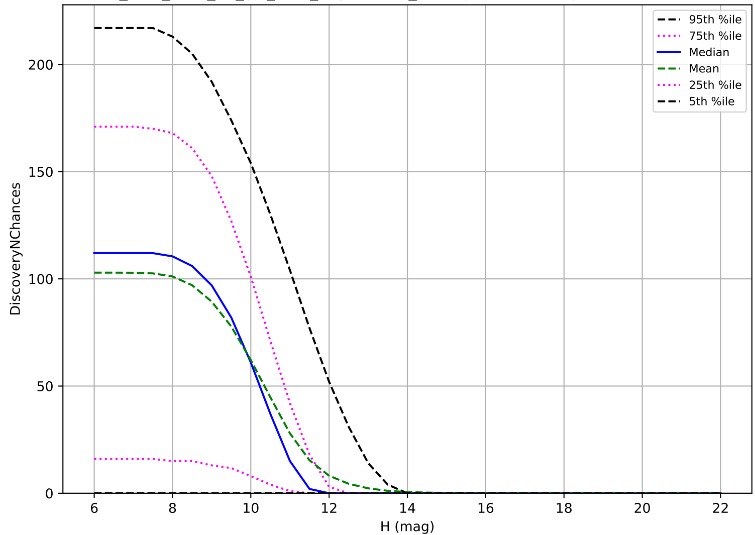
too_elab_r256_d3_giz_v3.4_10yrs: OCC_r20 3 pairs in 15 nights detection loss
