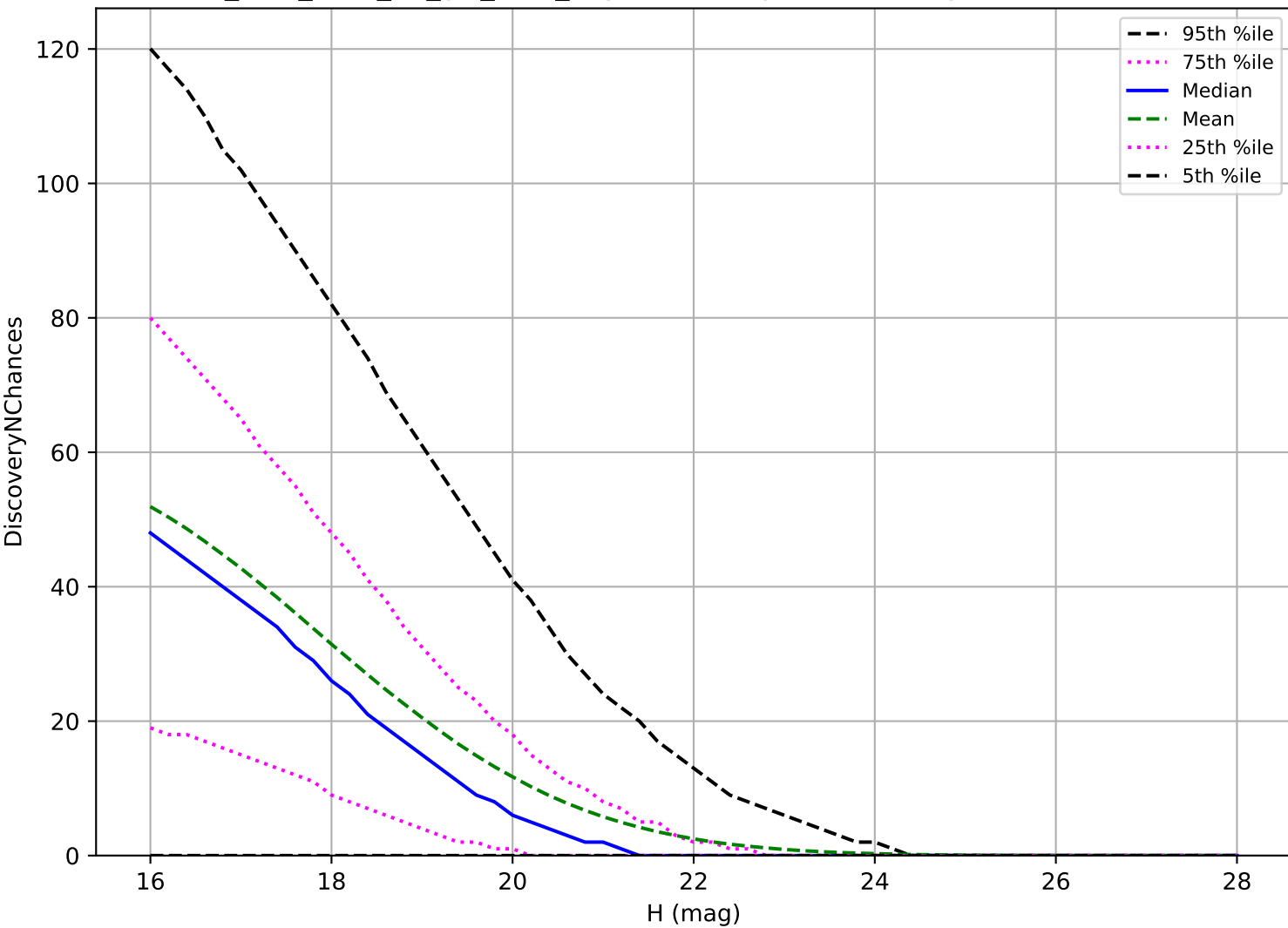
too_elab_r256_d3_giz_v3.4_10yrs: NEO 3 pairs in 15 nights detection loss
