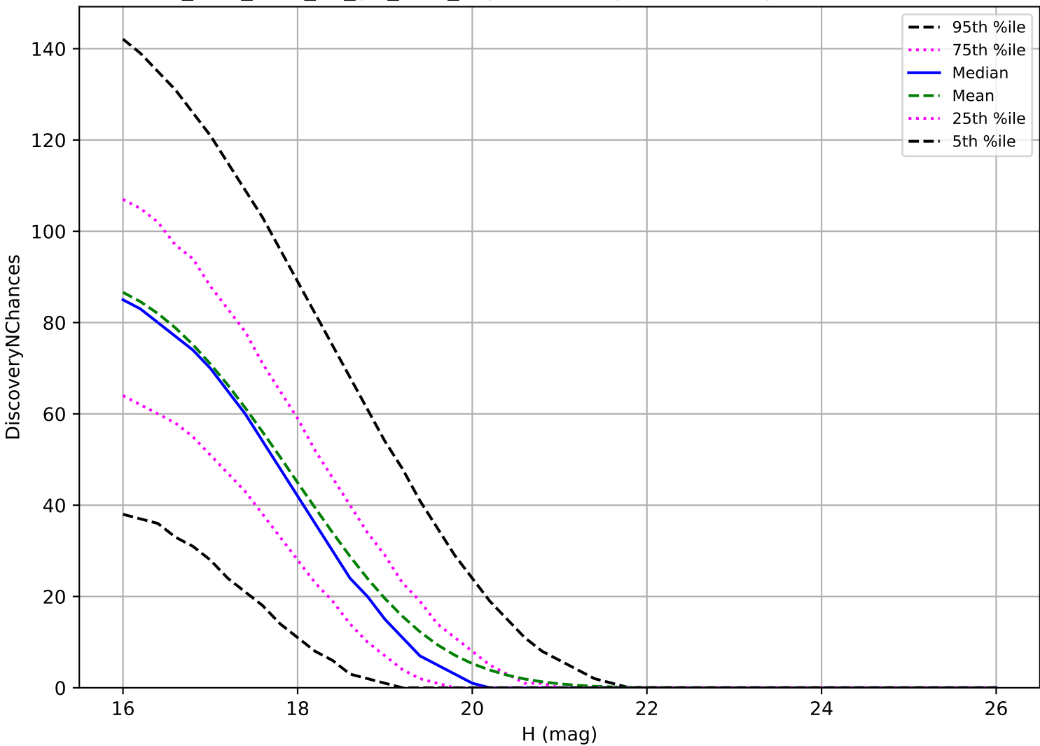
too_elab_r256_d3_giz_v3.4_10yrs: MBA 3 pairs in 15 nights detection loss
