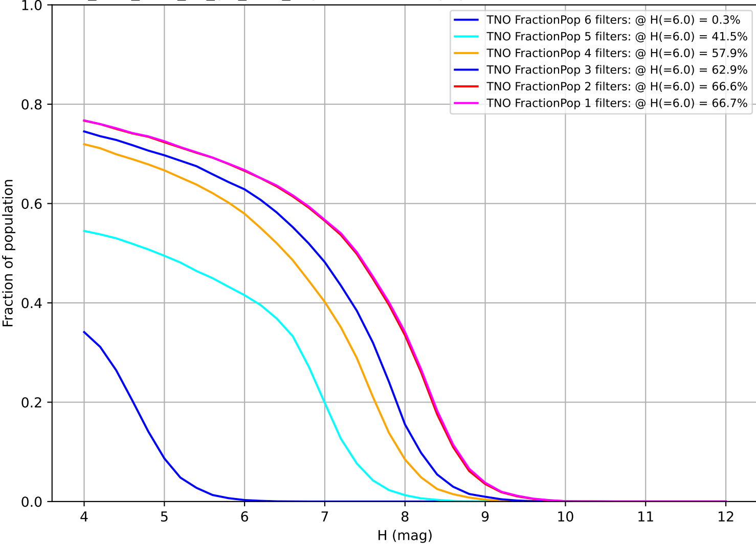
too_elab_r256_d3_giz_v3.4_10yrs: Fraction of population with colors in X filters TNO
