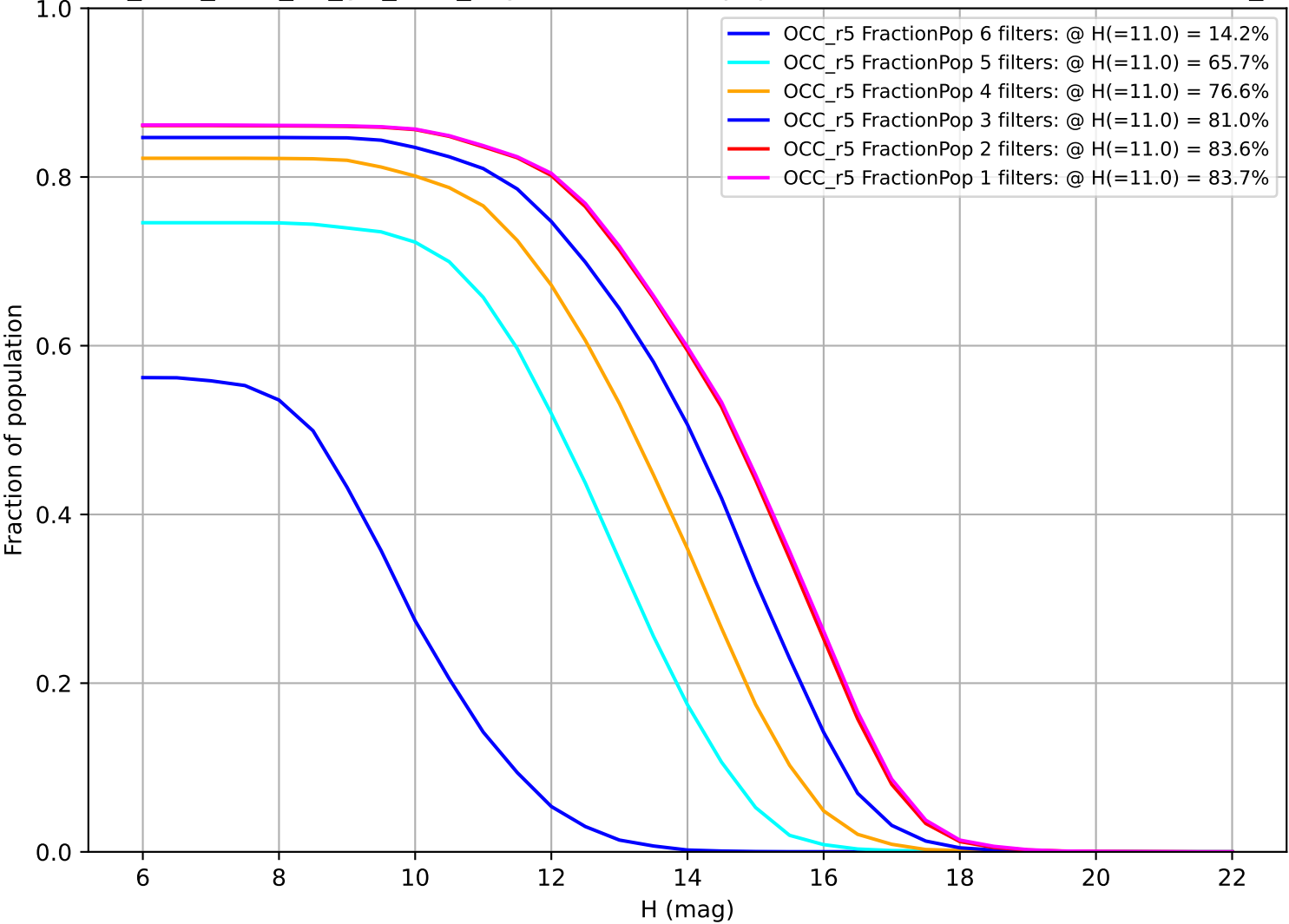
too_elab_r256_d3_giz_v3.4_10yrs: Fraction of population with colors in X filters OCC_r5
