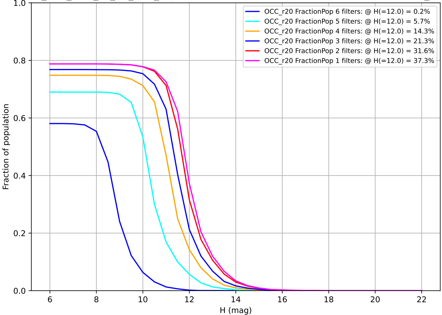
too_elab_r256_d3_giz_v3.4_10yrs: Fraction of population with colors in X filters OCC_r20
