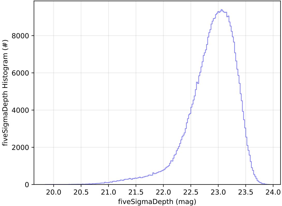
too_elab_r256_d3_giz_v3.4_10yrs z: fiveSigmaDepth Histogram
