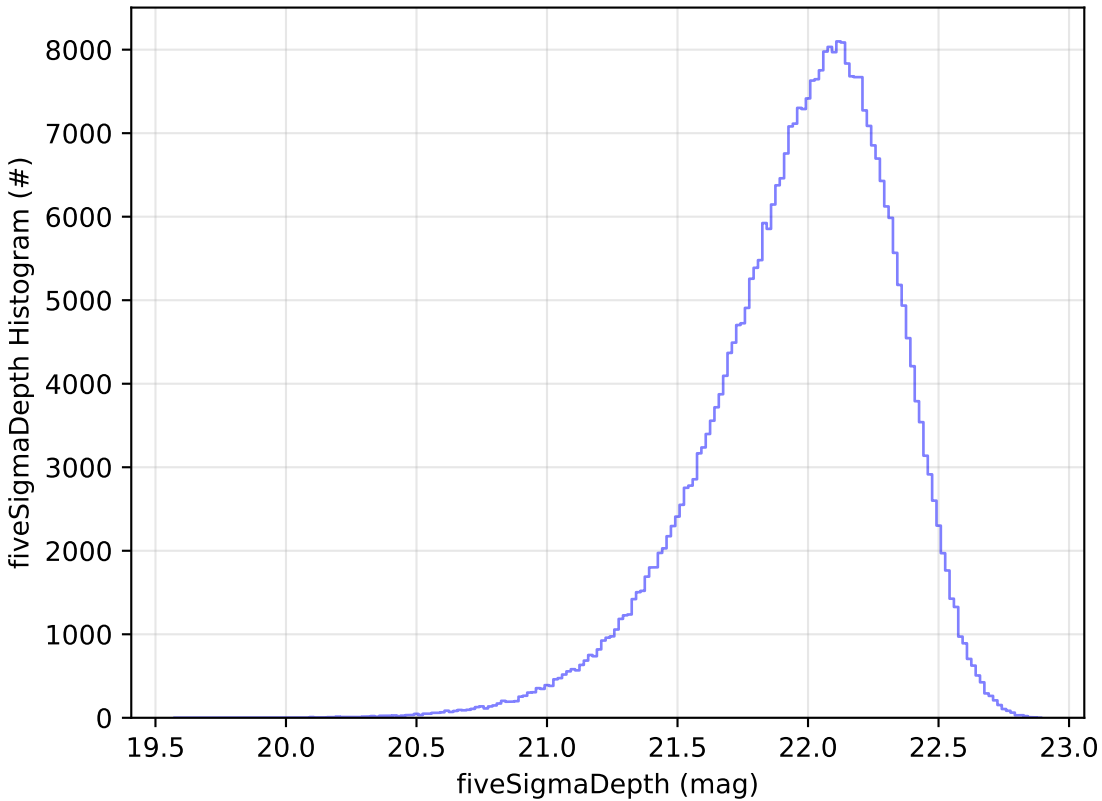
too_elab_r256_d3_giz_v3.4_10yrs y: fiveSigmaDepth Histogram
