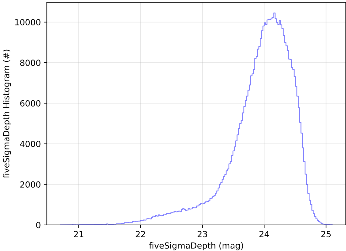
too_elab_r256_d3_giz_v3.4_10yrs r: fiveSigmaDepth Histogram
