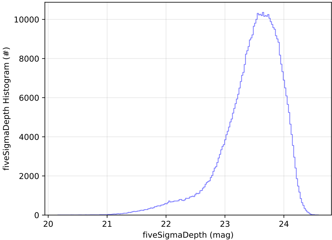
too_elab_r256_d3_giz_v3.4_10yrs i: fiveSigmaDepth Histogram
