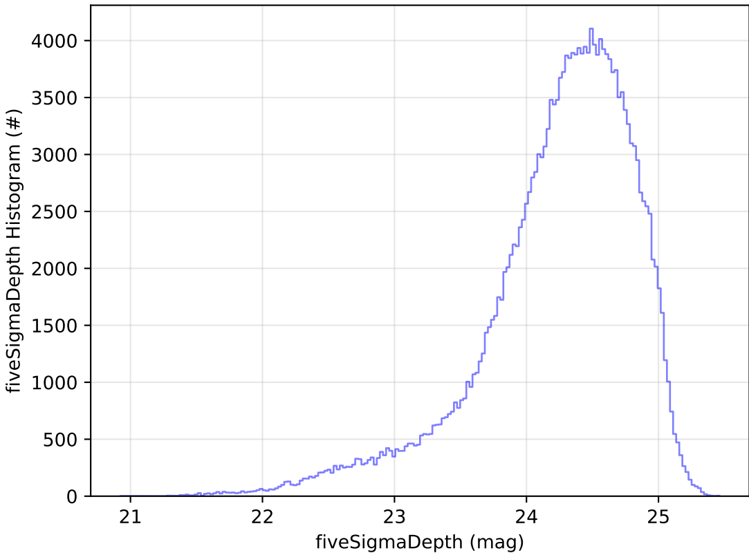
too_elab_r256_d3_giz_v3.4_10yrs g: fiveSigmaDepth Histogram
