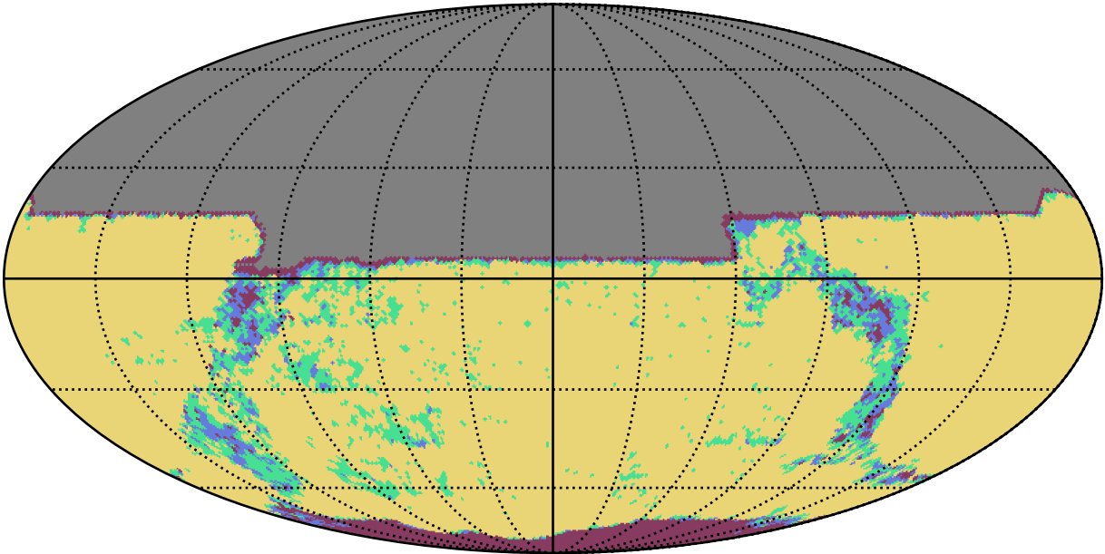
too_elab_r256_d3_giz_v3.4_10yrs y band: YearCoverage night
