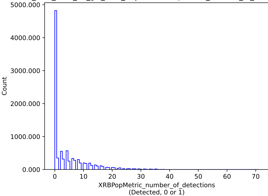
too_elab_r256_d3_giz_v3.4_10yrs : XRBPopMetric_number_of_detections
