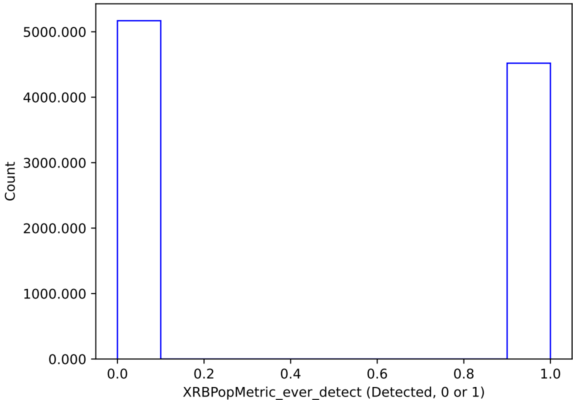
too_elab_r256_d3_giz_v3.4_10yrs : XRBPoMetric_ever_detect
