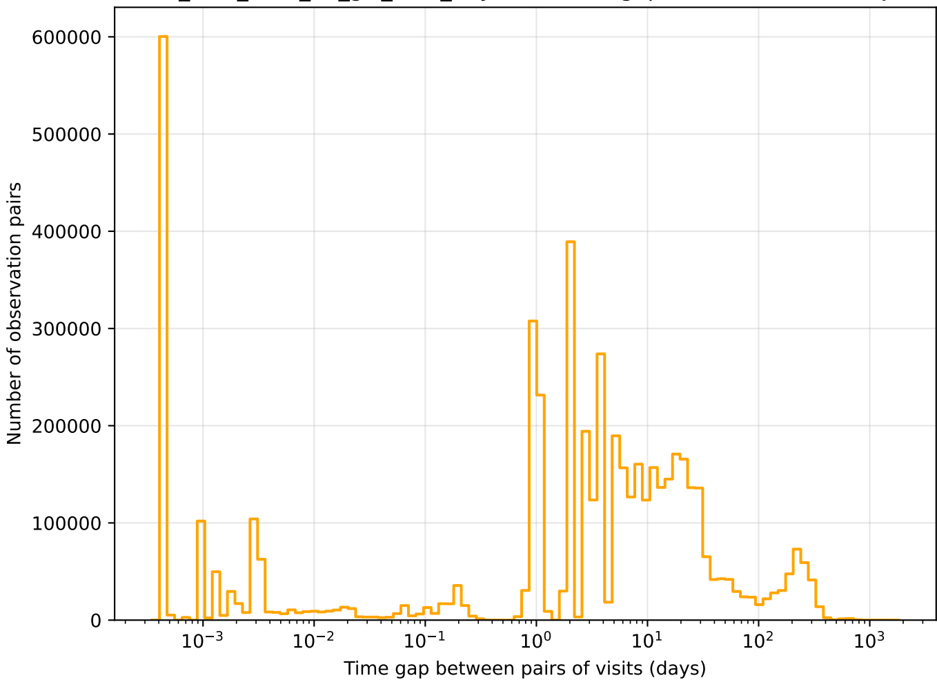
too_elab_r256_d3_giz_v3.4_10yrs r band: Tgaps observationStartMJD
