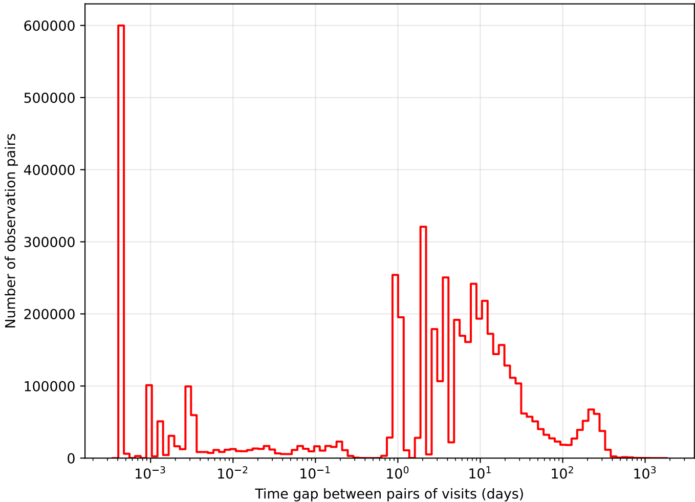
too_elab_r256_d3_giz_v3.4_10yrs i band: Tgaps observationStartMJD
