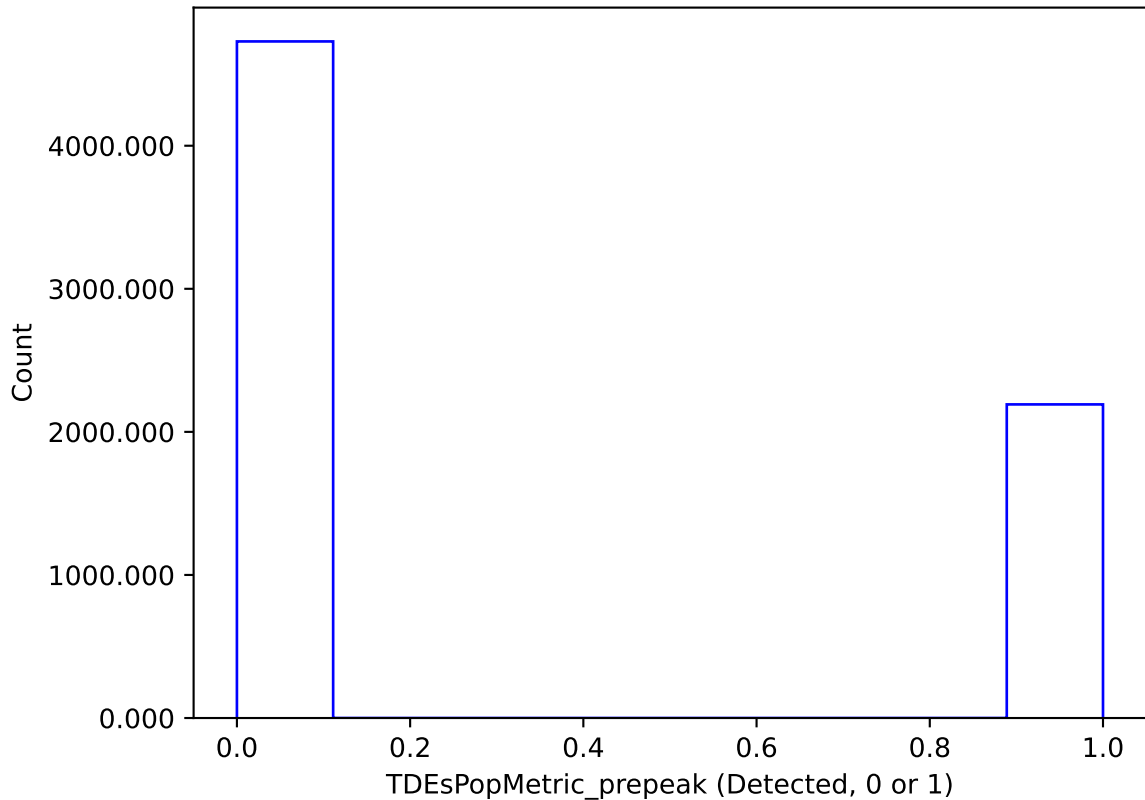
too_elab_r256_d3_giz_v3.4_10yrs : TDEsPopMetric_prepeak
