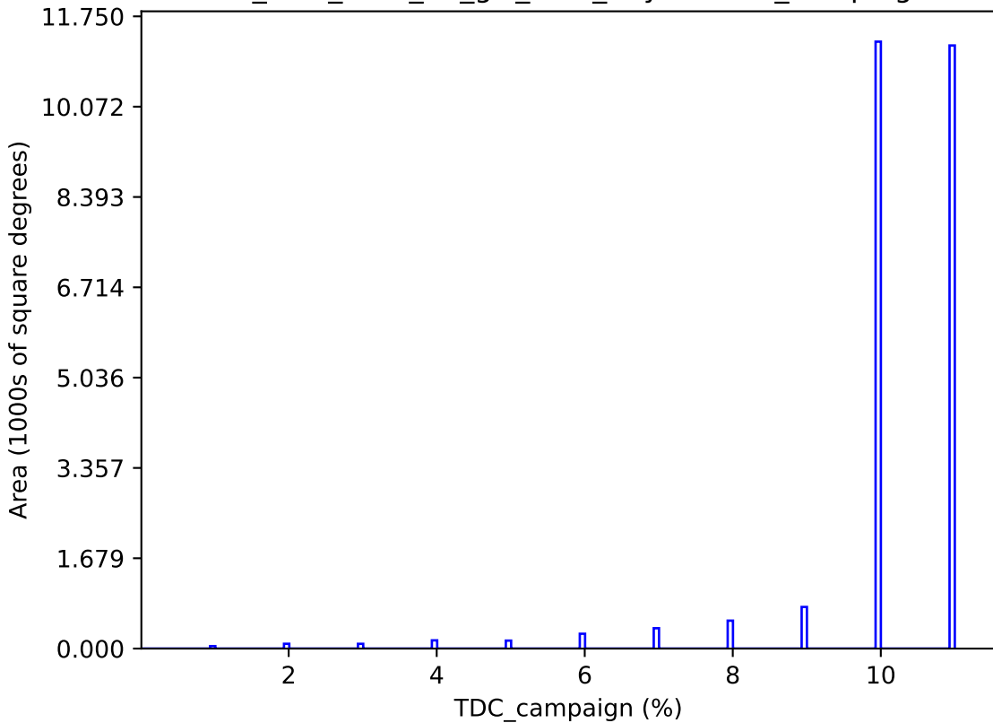
too_elab_r256_d3_giz_v3.4_10yrs : TDC_campaign
