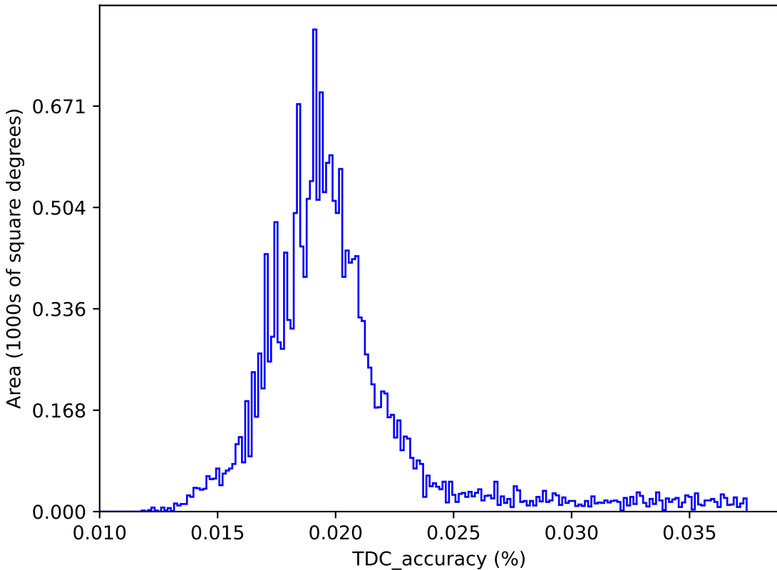
too_elab_r256_d3_giz_v3.4_10yrs : TDC_accuracy
