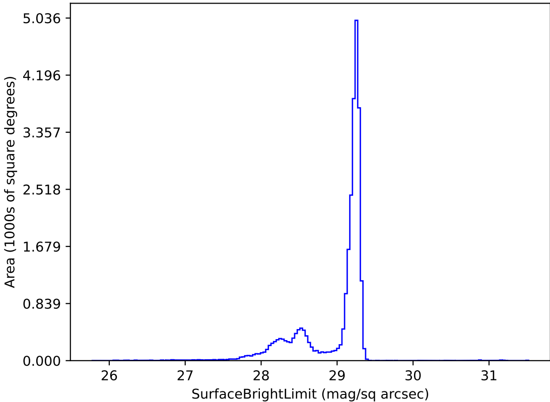
too_elab_r256_d3_giz_v3.4_10yrs z: SurfaceBrightLimit
