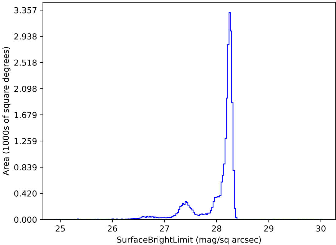
too_elab_r256_d3_giz_v3.4_10yrs y: SurfaceBrightLimit
