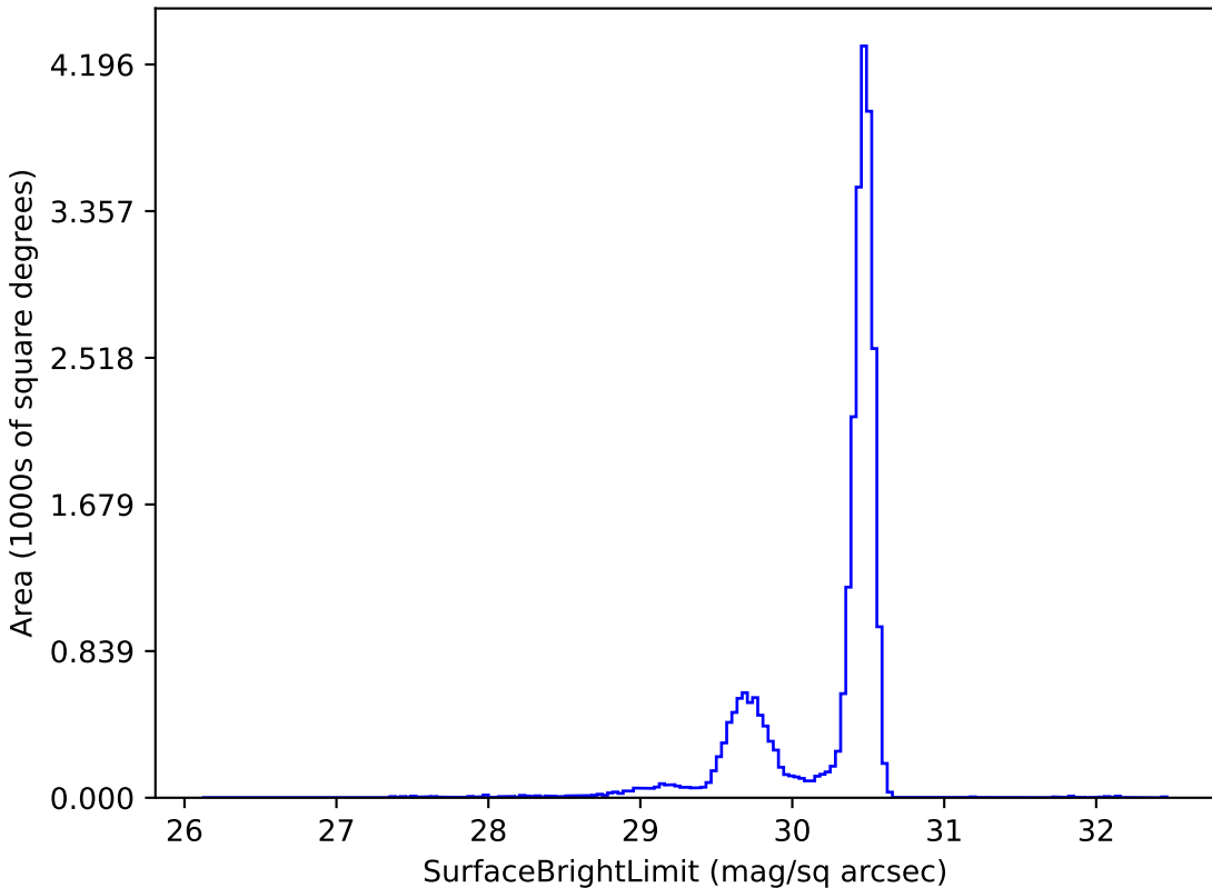
too_elab_r256_d3_giz_v3.4_10yrs r: SurfaceBrightLimit
