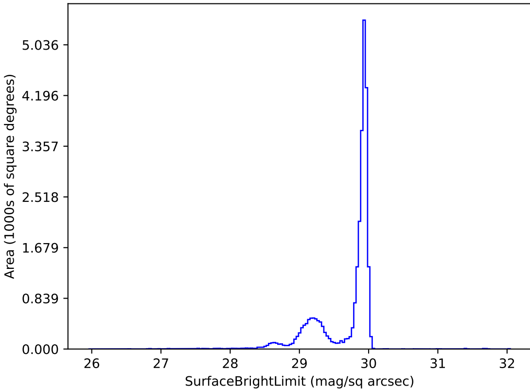
too_elab_r256_d3_giz_v3.4_10yrs i: SurfaceBrightLimit
