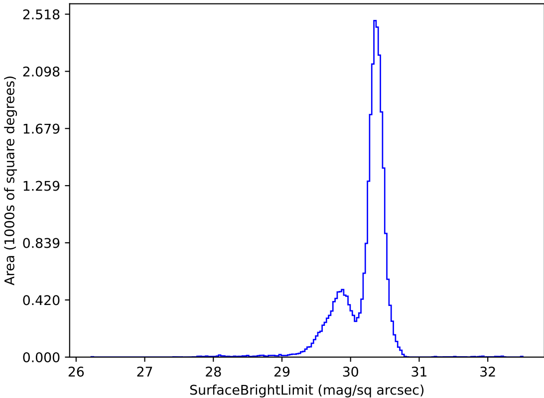
too_elab_r256_d3_giz_v3.4_10yrs g: SurfaceBrightLimit
