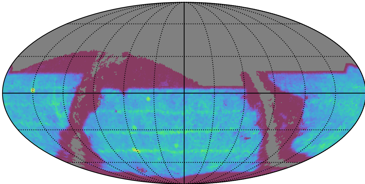
too_elab_r256_d3_giz_v3.4_10yrs : SNSLMetric
