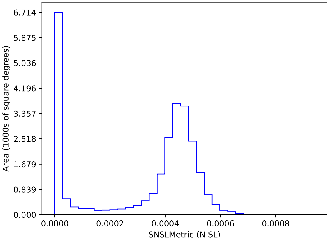
too_elab_r256_d3_giz_v3.4_10yrs : SNSLMetric
