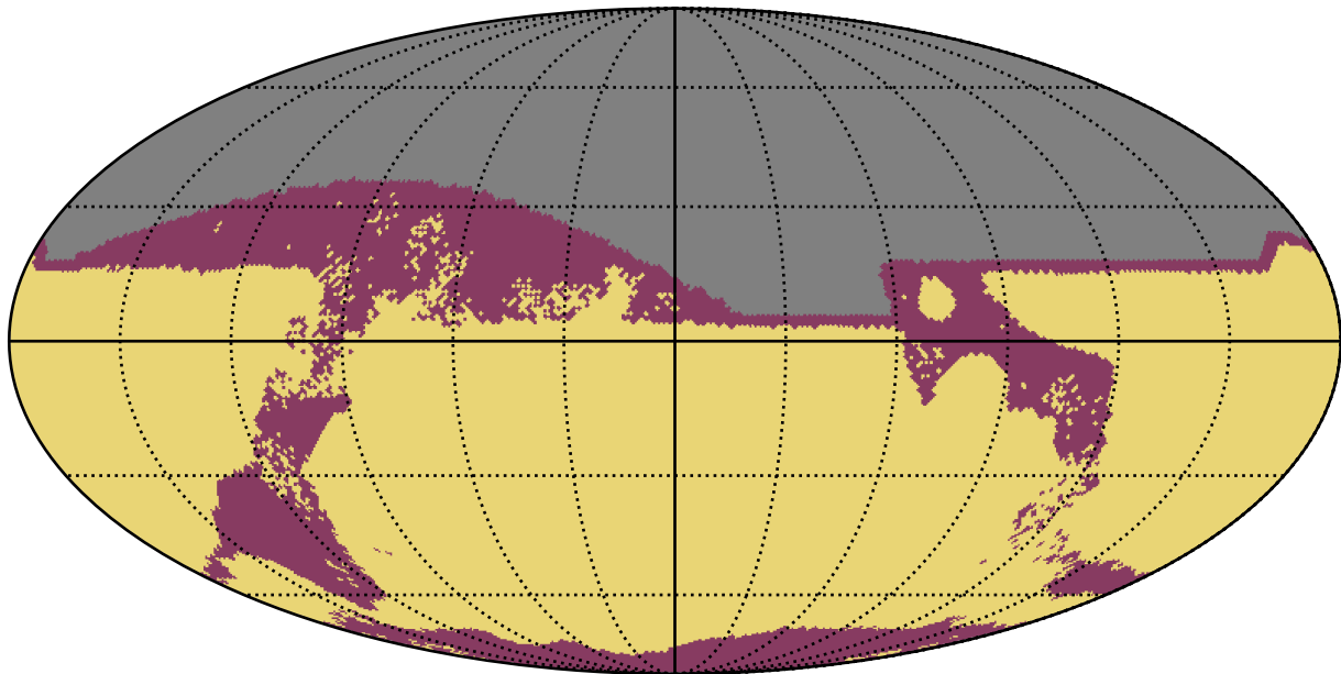
too_elab_r256_d3_giz_v3.4_10yrs : RapidRevisits
