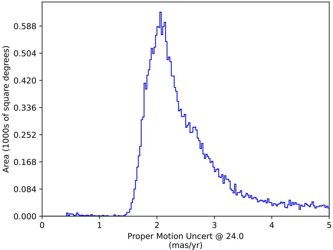
too_elab_r256_d3_giz_v3.4_10yrs : Proper Motion Uncert @ 24.0
