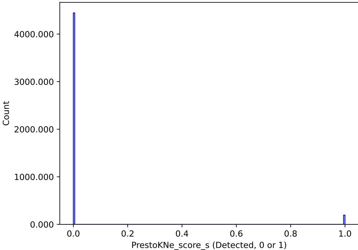
too_elab_r256_d3_giz_v3.4_10yrs : PrestoKNe_score_s
