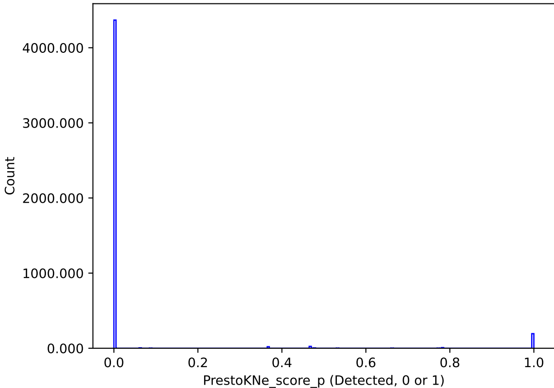
too_elab_r256_d3_giz_v3.4_10yrs : PrestoKNe_score_p
