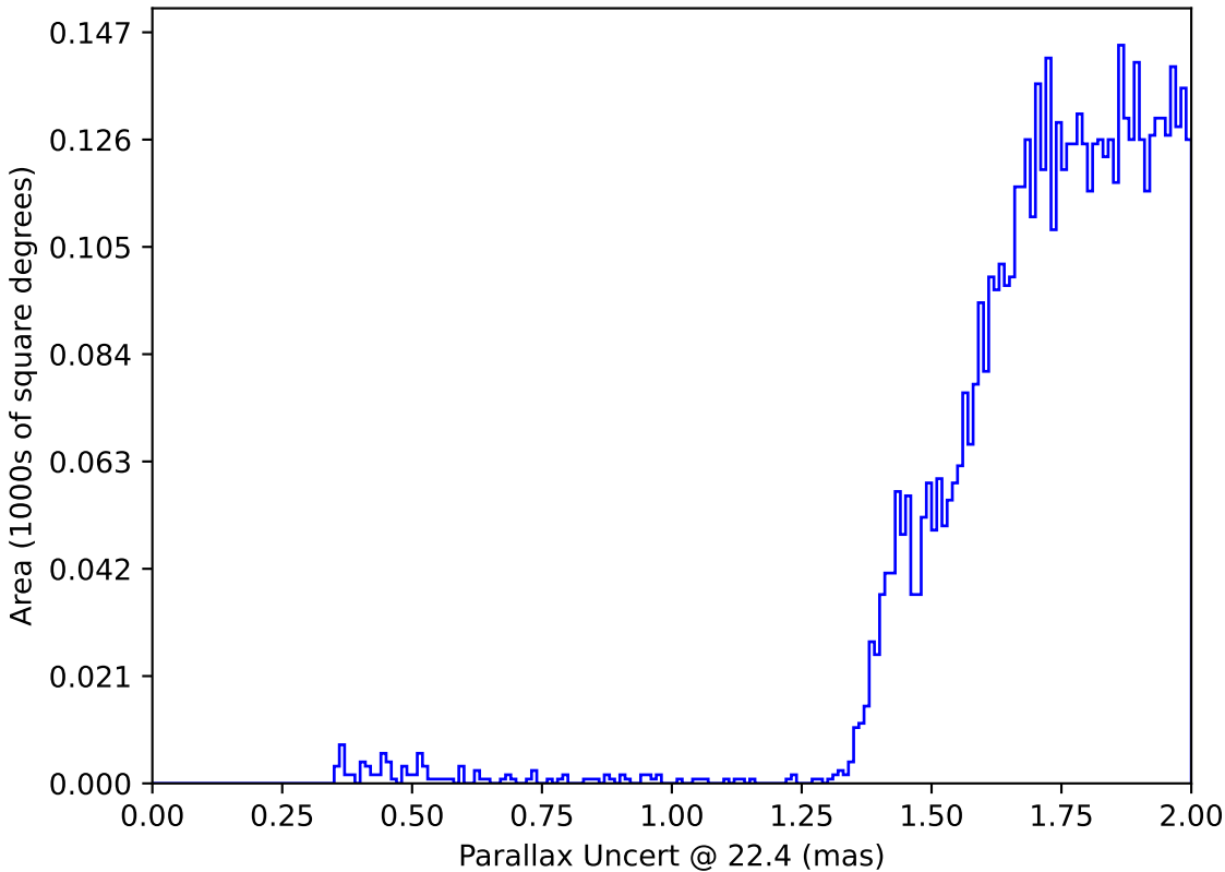
too_elab_r256_d3_giz_v3.4_10yrs : Parallax Uncert @ 22.4
