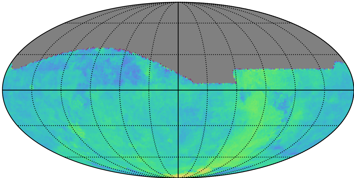
too_elab_r256_d3_giz_v3.4_10yrs : Parallax Coverage @ 24.0
