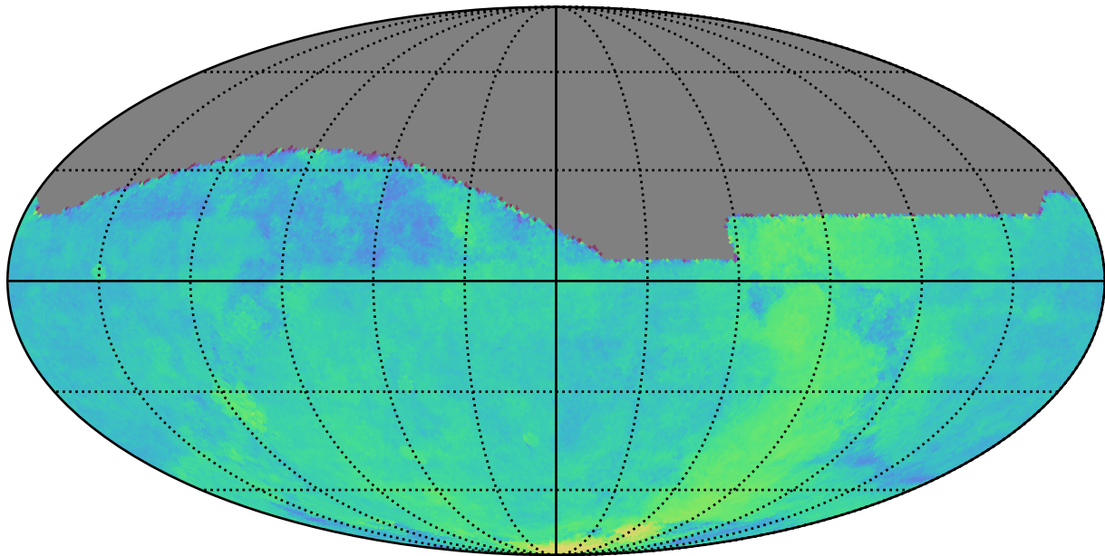
too_elab_r256_d3_giz_v3.4_10yrs : Parallax Coverage @ 22.4
