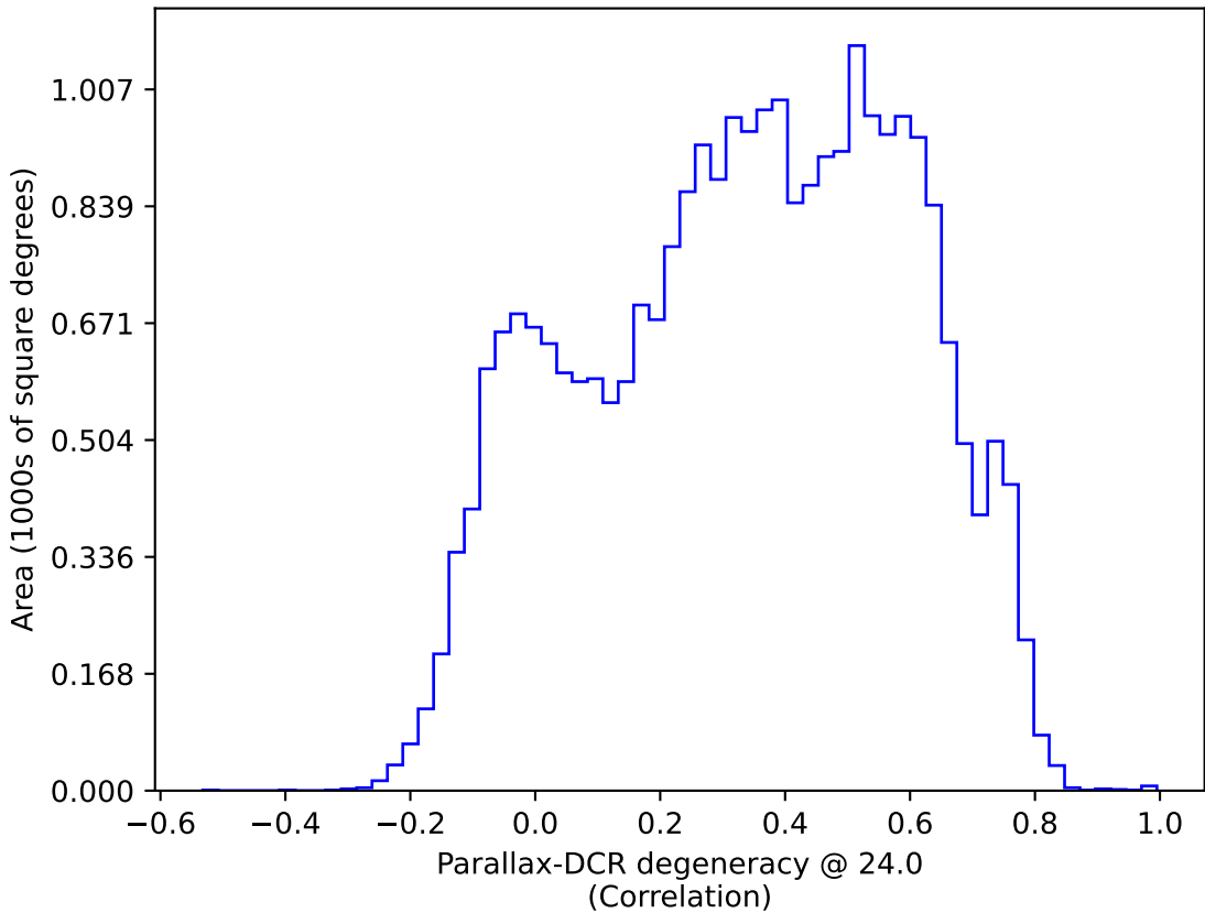
too_elab_r256_d3_giz_v3.4_10yrs : Parallax-DCR degeneracy @ 24.0
