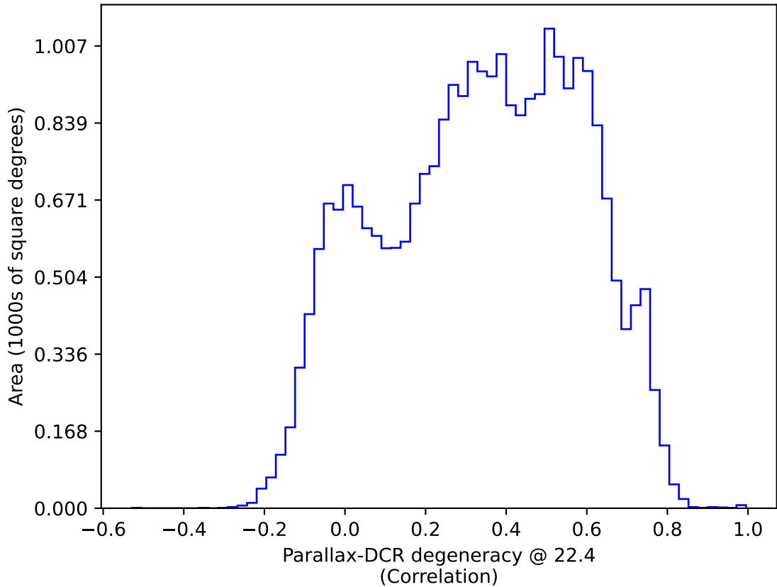
too_elab_r256_d3_giz_v3.4_10yrs : Parallax-DCR degeneracy @ 22.4
