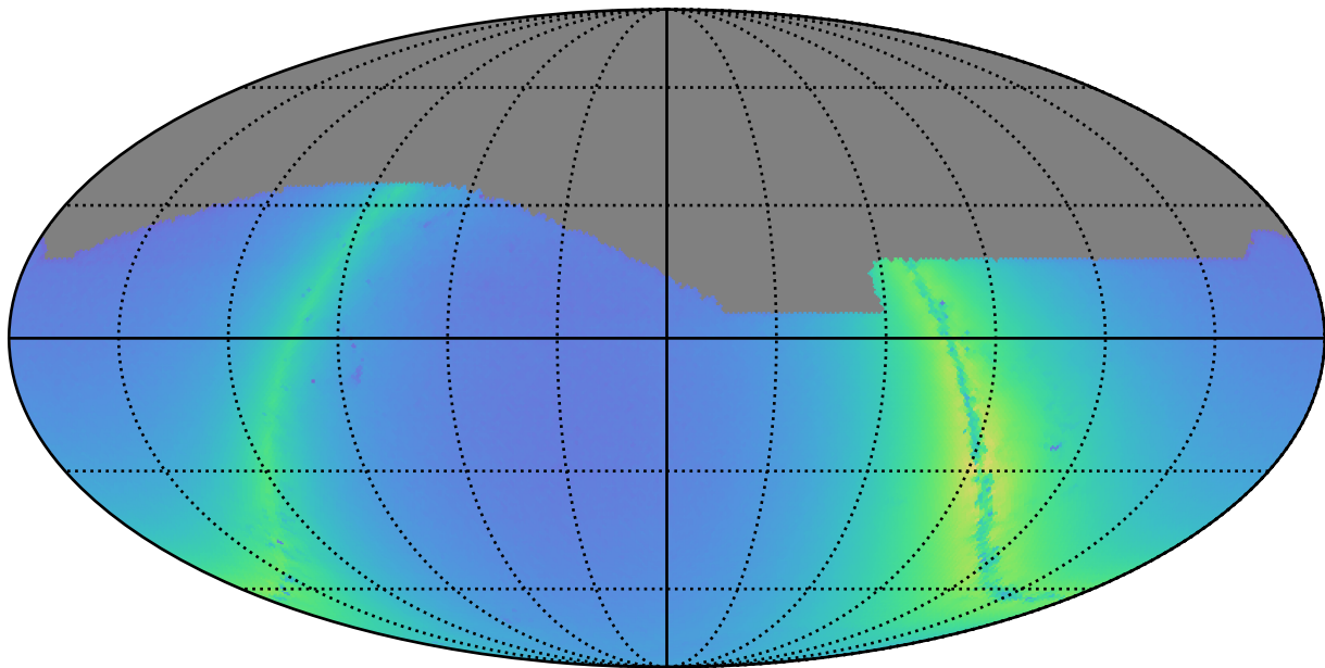
too_elab_r256_d3_giz_v3.4_10yrs i: Nstars_no_crowding
