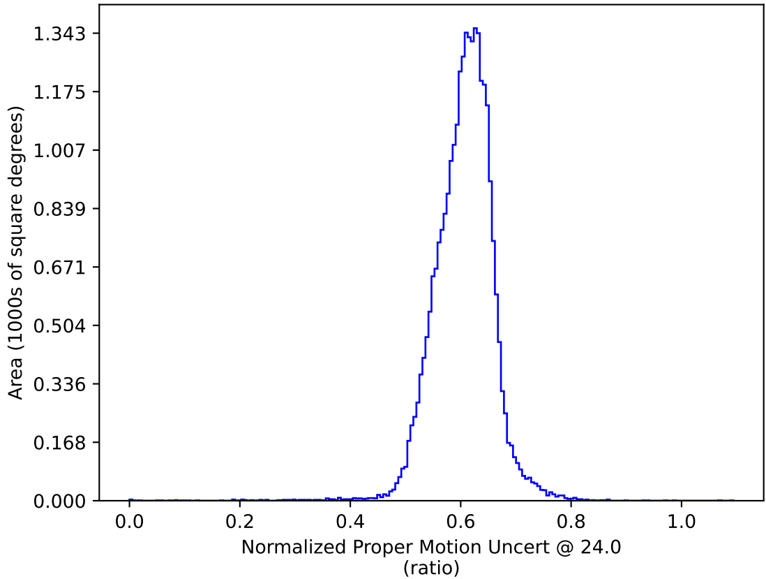
too_elab_r256_d3_giz_v3.4_10yrs : Normalized Proper Motion Uncert @ 24.0
