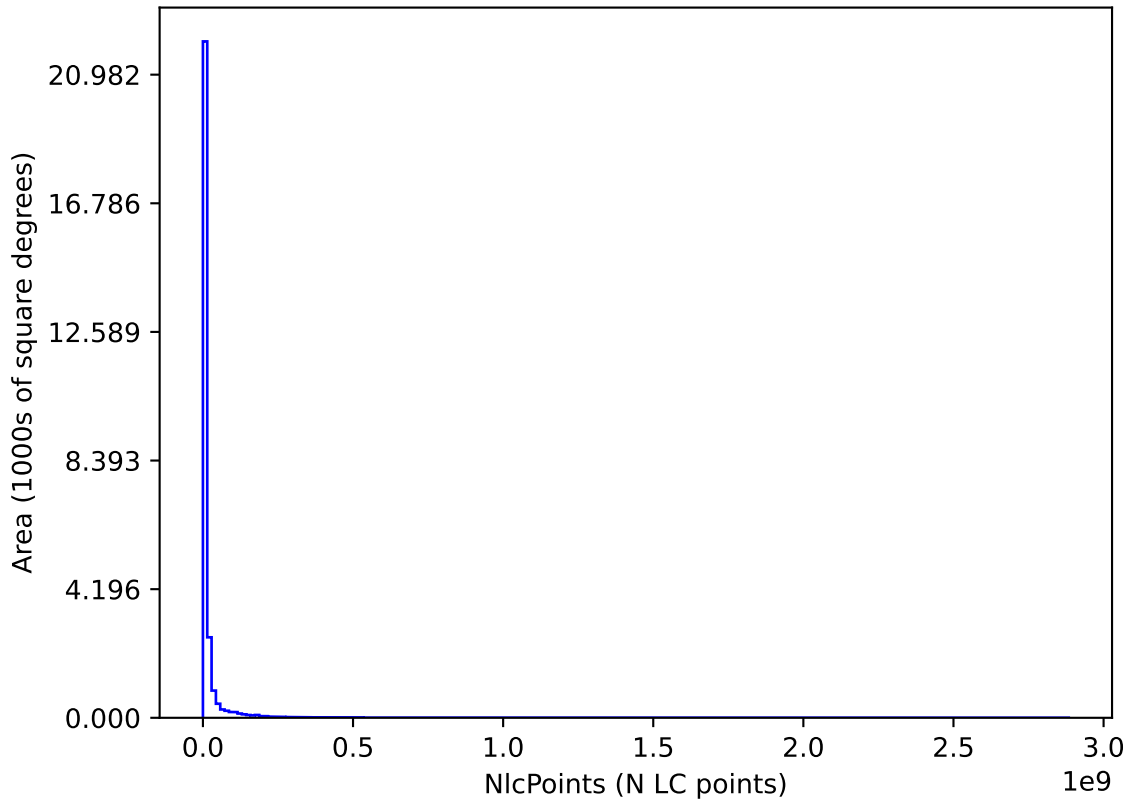
too_elab_r256_d3_giz_v3.4_10yrs : NlcPoints
