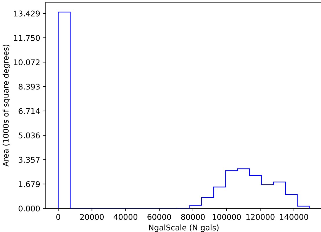
too_elab_r256_d3_giz_v3.4_10yrs i: NgalScale
