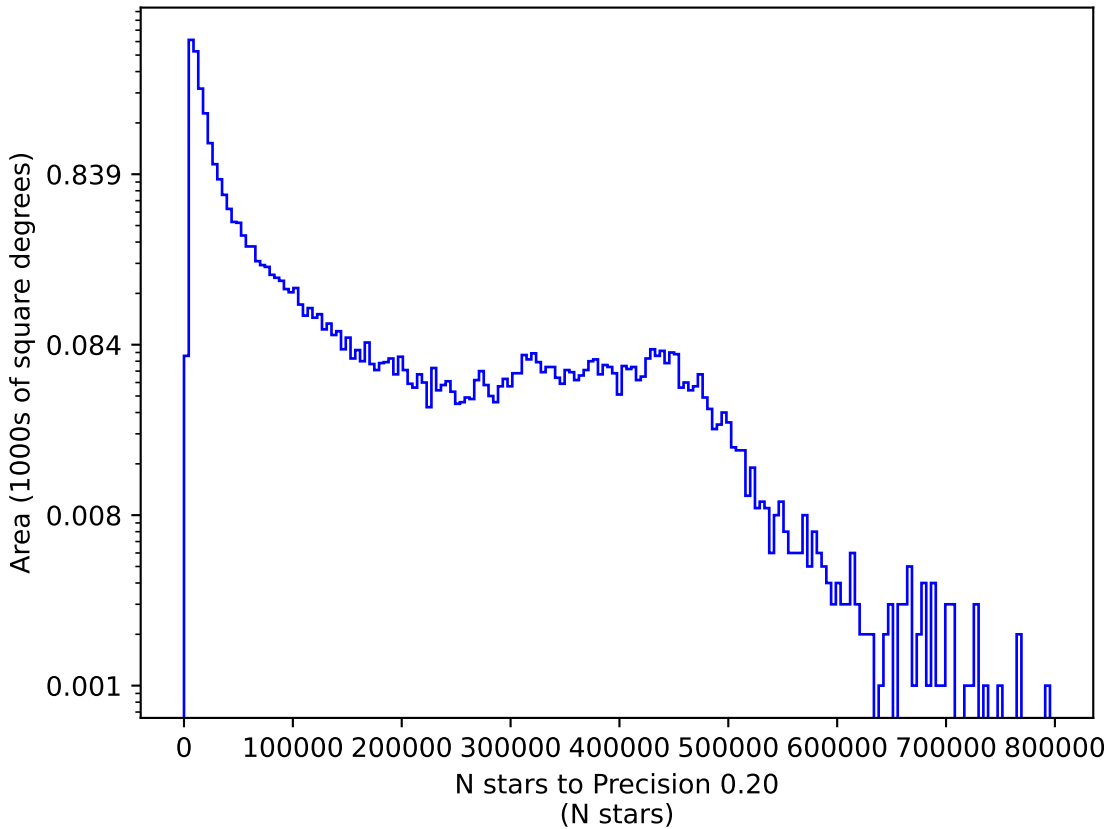
too_elab_r256_d3_giz_v3.4_10yrs r: N stars to Precision 0.20
