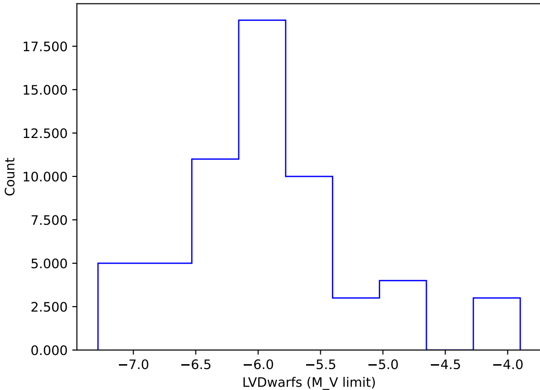
too_elab_r256_d3_giz_v3.4_10yrs gi: LVDwarfs
