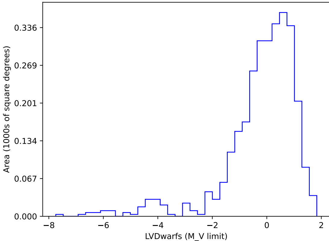
too_elab_r256_d3_giz_v3.4_10yrs gi SCP: LVDwarfs
