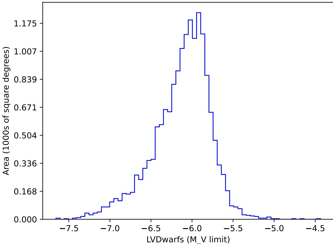
too_elab_r256_d3_giz_v3.4_10yrs gi: LVDwarfs
